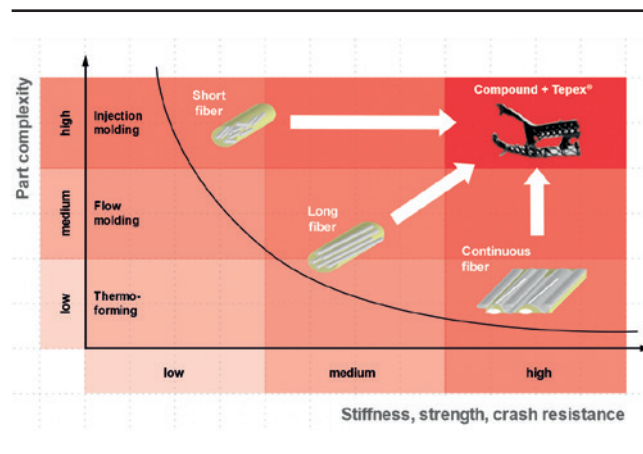
Figure 9: Diagram of combination options for Tepex® with compounds
